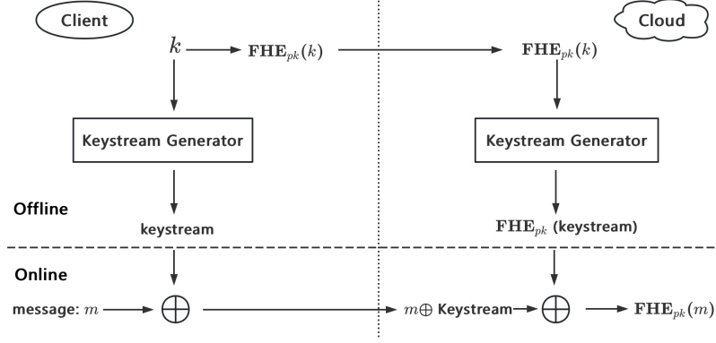
Figure 1: Transciphering framework based on stream cipher.
